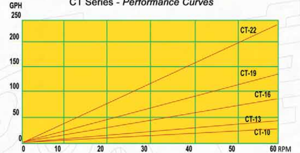
CT Series - Performance Curves
