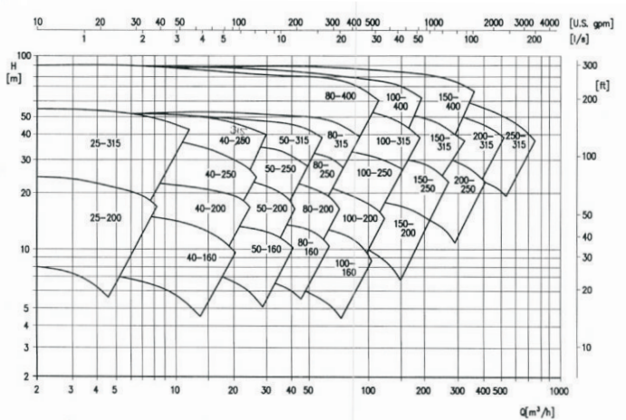
N=1800 rpm 60 Hz
