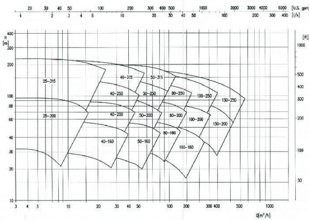
N=3600 rpm 60 Hz
