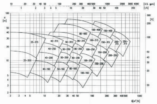
N=1500 rpm 50 Hz
